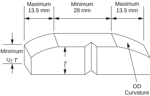
Figure F-1—Impact Test Specimen Tapered End Allowance
