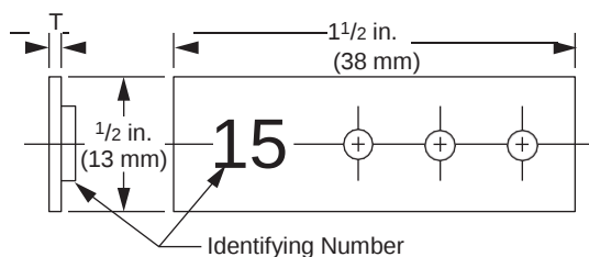
Figure 5—Flattening Tests
